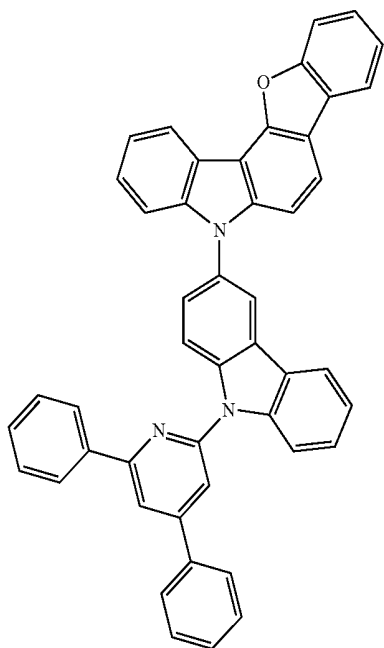
[Chemical Formula B-3]
