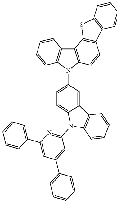
[Chemical Formula A-3]
