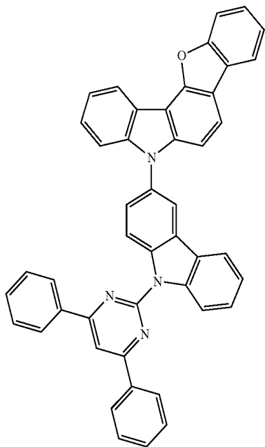
[Chemical Formula B-2]
