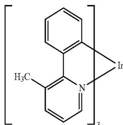
[PhGD]
