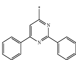
[Chemical Formula 8]
