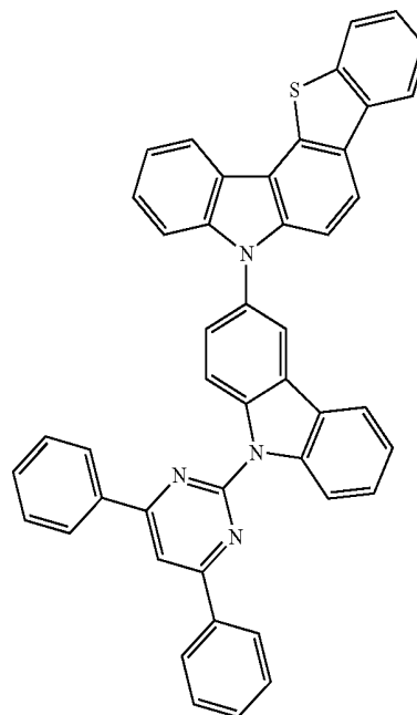
[Chemical Formula A-2]
