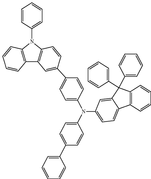
[HTM]
