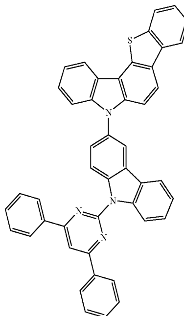
[Chemical Formula A-2]
