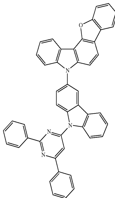
[Chemical Formula B-4]
