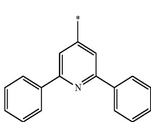
[Chemical Formula 9]
