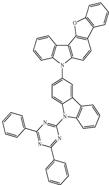
[Chemical Formula B-1]
