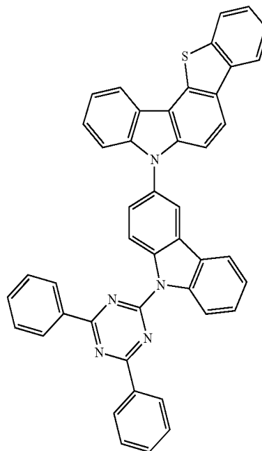
[Chemical Formula A-1]
