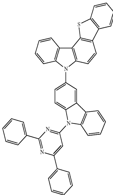
[Chemical Formula A-4]
