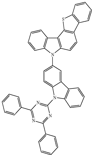
[Chemical Formula A-1]
